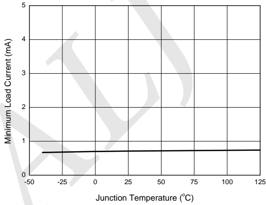
Figure 6. Minimum Load Current vs. Junction Temperature
